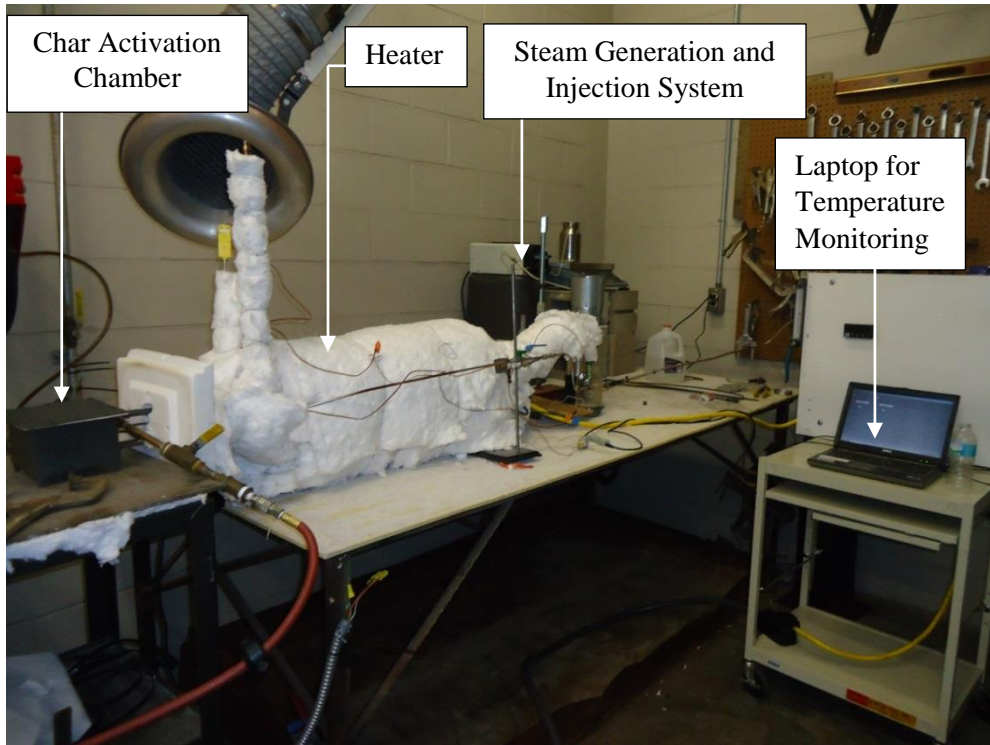
Figure: char activation system
