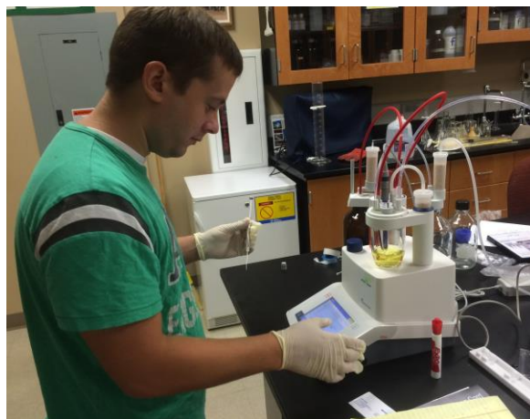
Figure: Determination of water of pyrolysis using K-F titrator
