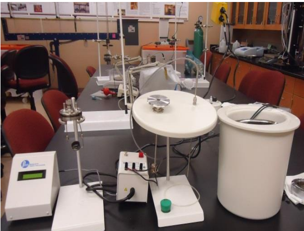
Lab Tests: HHV Determination (Calorimeter)
