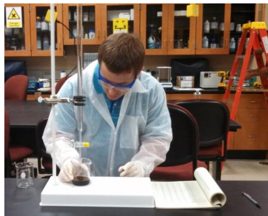
Lab Tests: Iodine Number Determination (Titration)
